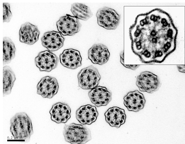
FIGURE 3 Electron microscopy image of normal ciliary ultrastructure from an Irish Wolfhound with recurrent bacterial pneumonia. Cilia exhibit correct number and shape of central and peripheral doublets, spikes and dynein arms
